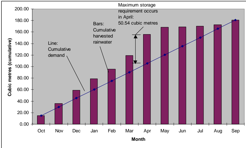
Figure 11: showing the predicted cumulative inflow and outflow from the tank. The maximum storage requirement occurs in April at 50.54 cubic metres. All this water will have to be stored to cover the shortfall during the dry period.
